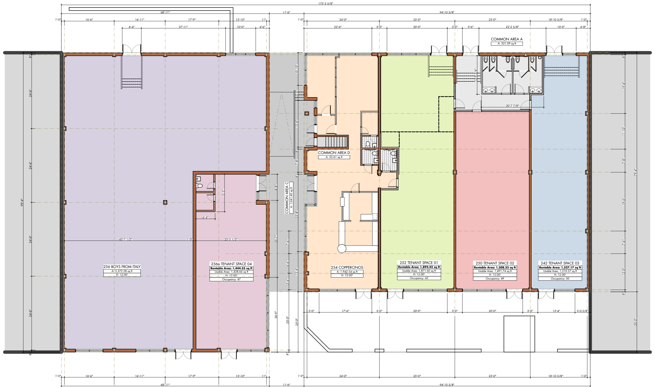
Floor Plan
